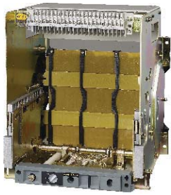
Drawer seat
